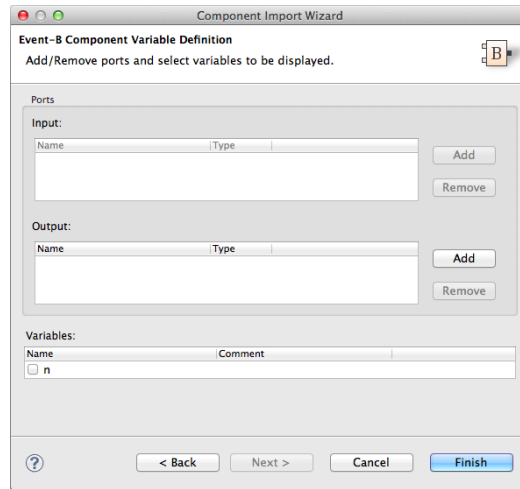
Figure 3.10: Event-B component variable definition page
