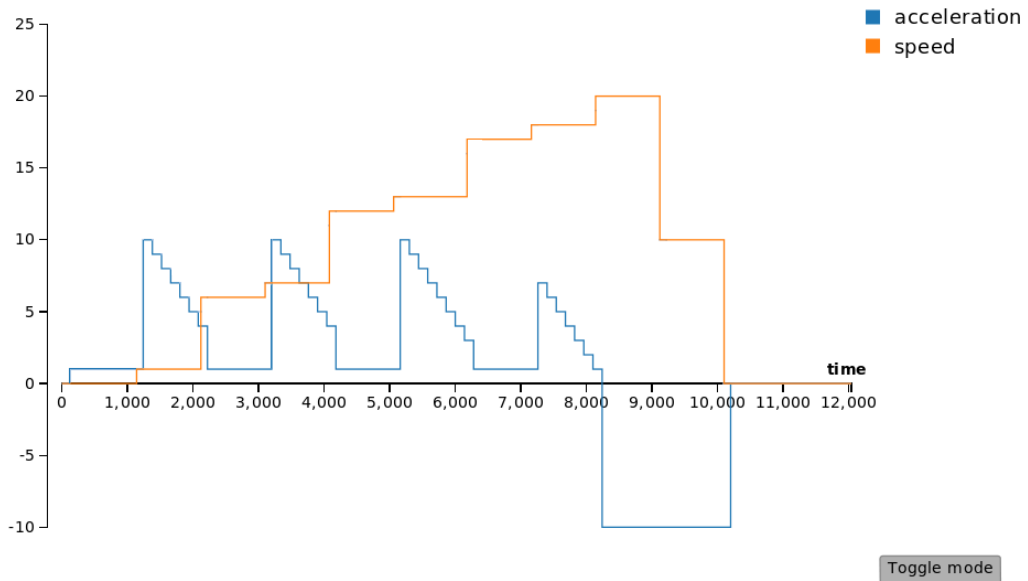
Figure 4.4: Value over time visualization
