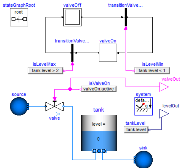
Figure 3.12: Controlled water tank model in Dymola
