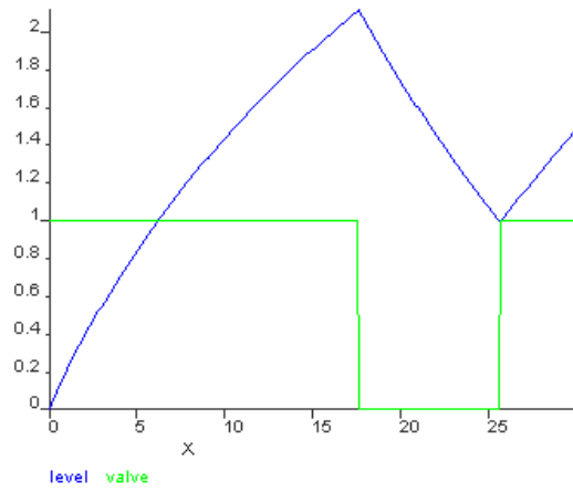
Figure 3.16: Co-simulation results of the controlled water tank model in the multi-simulation framework (simulation time = 30s, step size = 0.1s)
