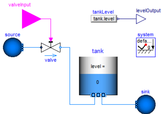
Figure 3.14: Controlled water tank plant subsystem
