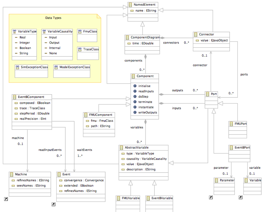
Figure 3.5: Metamodel of the co-simulation framework
