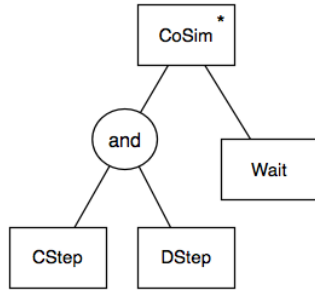
Figure 3.1: Abstract view of the co-simulation master
