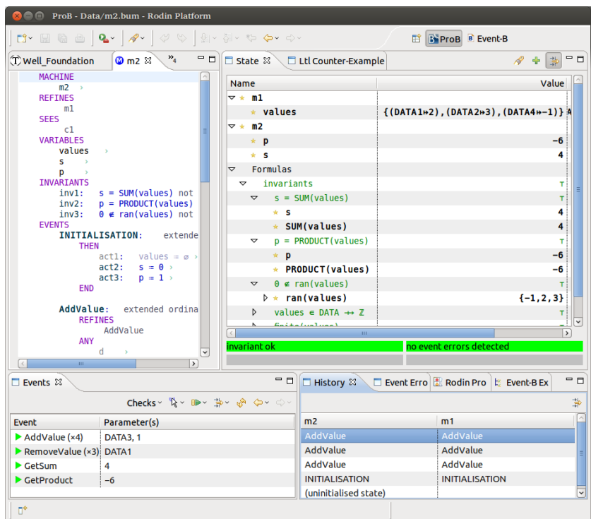
Figure 2.1: Screenshot of an animation using the theory of sum and product
