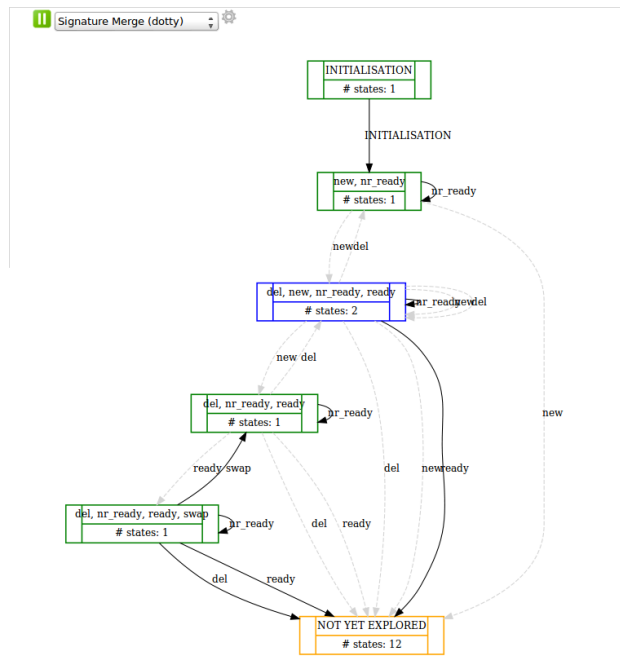
Figure 4.2: Reduced state space using the signature merge algorithm
