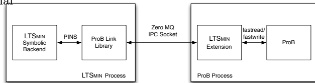
Fig. 8: High level design showing the integration
