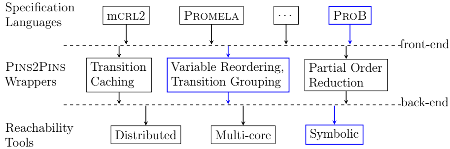
Fig. 1: Modular PINS architecture of LTSMIN [16]
