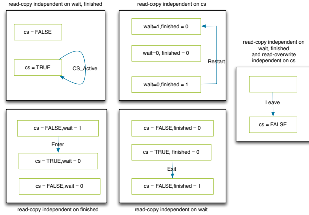
Fig. 6: MDDs of the reachable states
