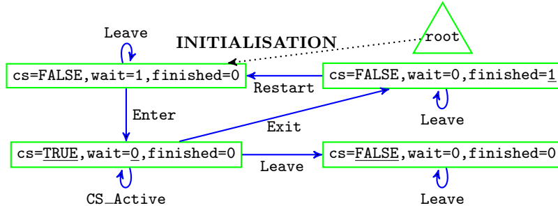
Fig. 3: MutexSimple statespace for MAXINT=1
